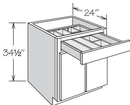
24" WITH ADJUSTABLE DIVIDER INSERT
