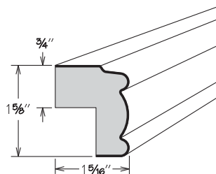
SMALL TRADITIONAL
