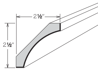
SMALL COVE
