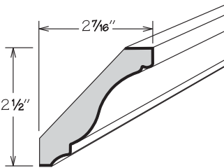
LARGE CROWN
