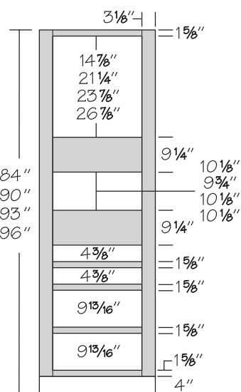
Single Oven Cabinet 4 Drawers*
