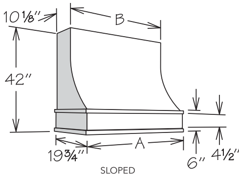
SLOPED
