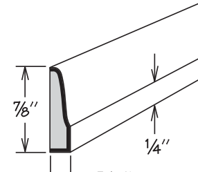
SHOE
