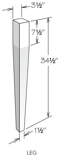
LEG
