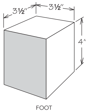
FOOT
