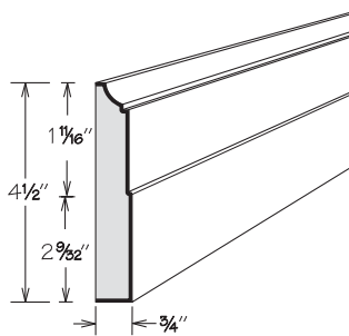
CLASSIC BASEBOARD
