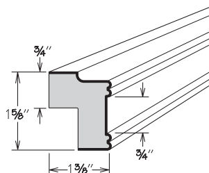
INSET
