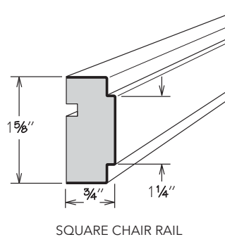
CHAIR RAIL CR8
