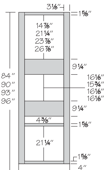
Single Oven Cabinet 1 Drawer*
