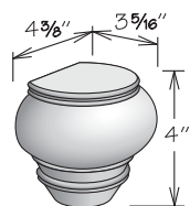
FOOT
