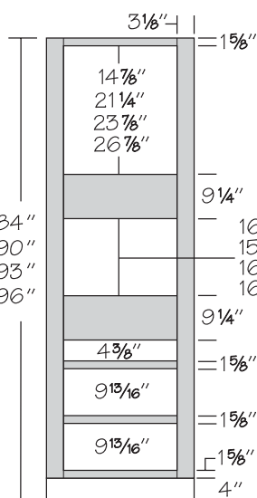
Single Oven Cabinet 3 Drawers*
