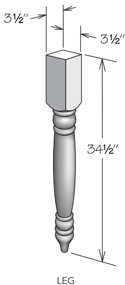
LEG
